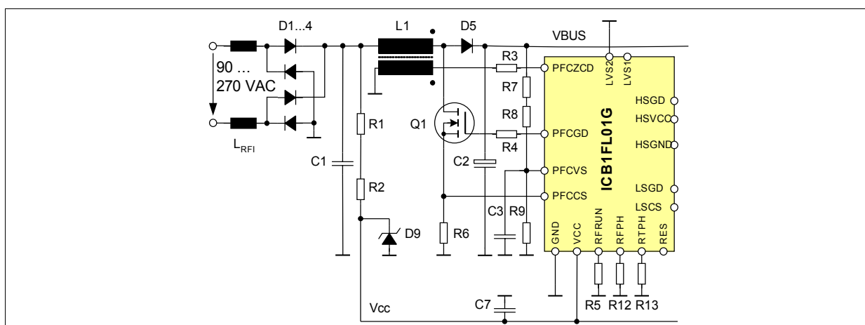
Figure 5 Circuit Diagram of the PFC preconverter section.
