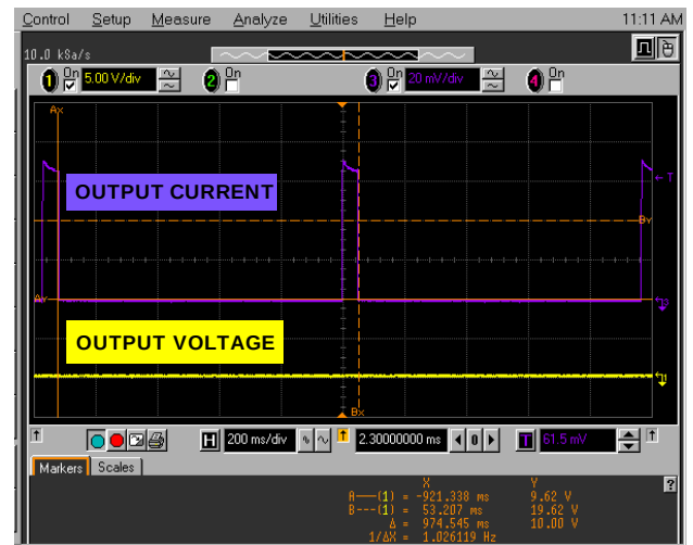
FIGURE 15. VLN SHORTED TO GND, 200mA 2
