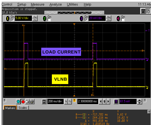
FIGURE 14. VLN CONNECTED TO 350mA LOAD WITH R_{ILIM} = 148k
