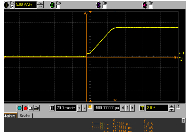
FIGURE 5. V_LNB RISE TIME WITH T_CAP = 0.44 \mu F is 32ms
