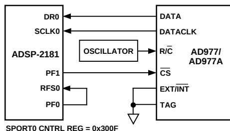
Figure 26. AD977/AD977A to ADSP-2181 Interface
