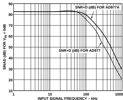
Figure 20. S/(N+D) vs. Input Frequency
