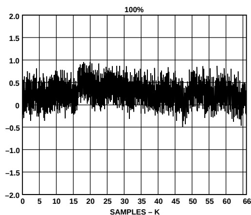
Figure 18. INL Plot
