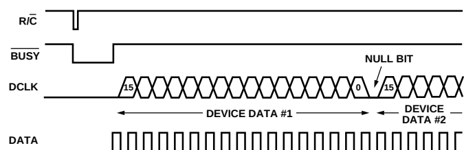
Figure 24. TAG Timing Diagram for Two Concatenated AD977/AD977As
