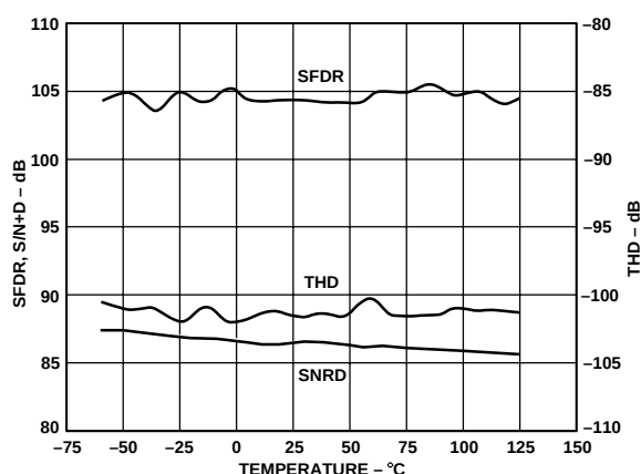
Figure 21. AC Parameters vs. Temperature
