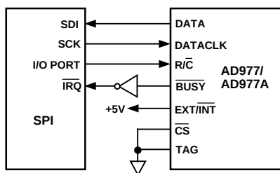
Figure 25. AD977/AD977A to SPI Interface
