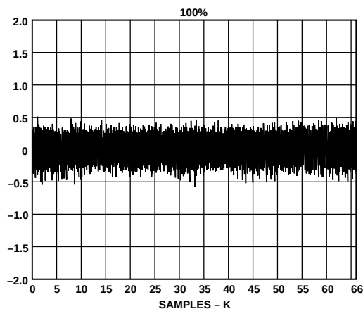
Figure 19. DNL Plot
