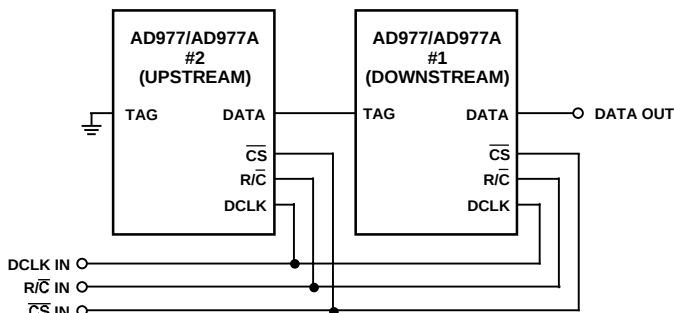
Figure 23. Two AD977/AD977A's Utilizing Tag
