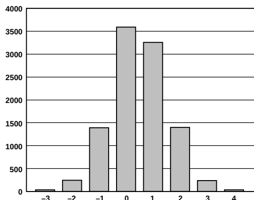
Figure 22. Histogram of 10,000 Conversions of a DC Input
