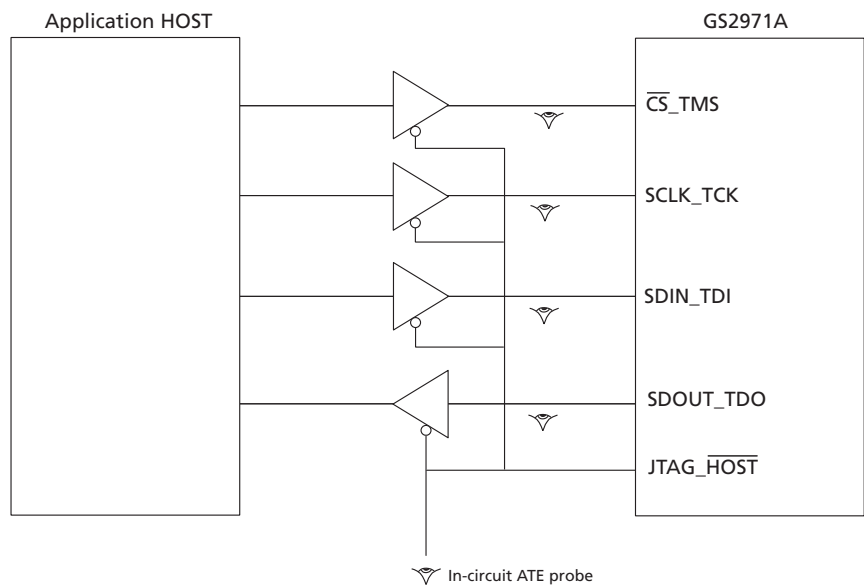
Figure 4-54: In-Circuit JTAG
