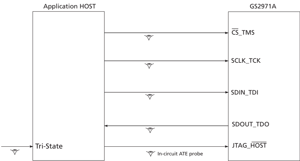
Figure 4-55: System JTAG
