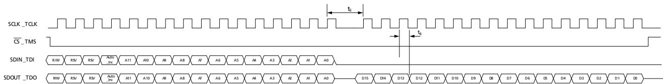
Figure 4-52:Read Mode
