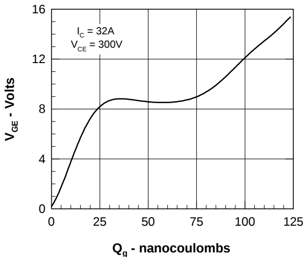
Fig. 9. Gate Charge
