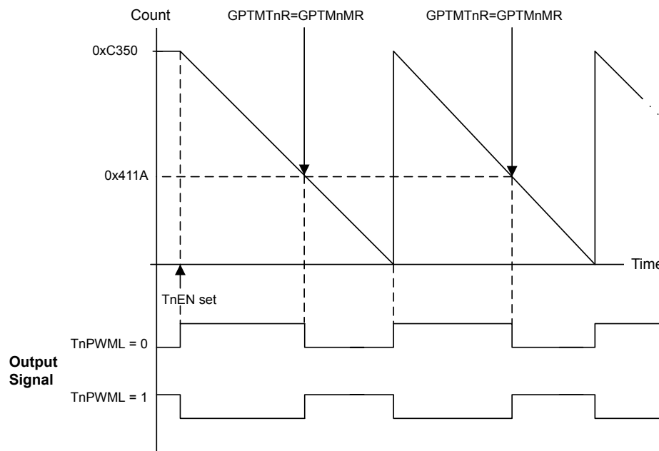
Figure 10-4. 16-Bit PWM Mode Example
