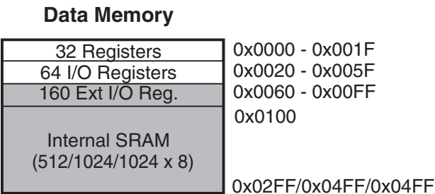
Figure 8-3. Data Memory Map
