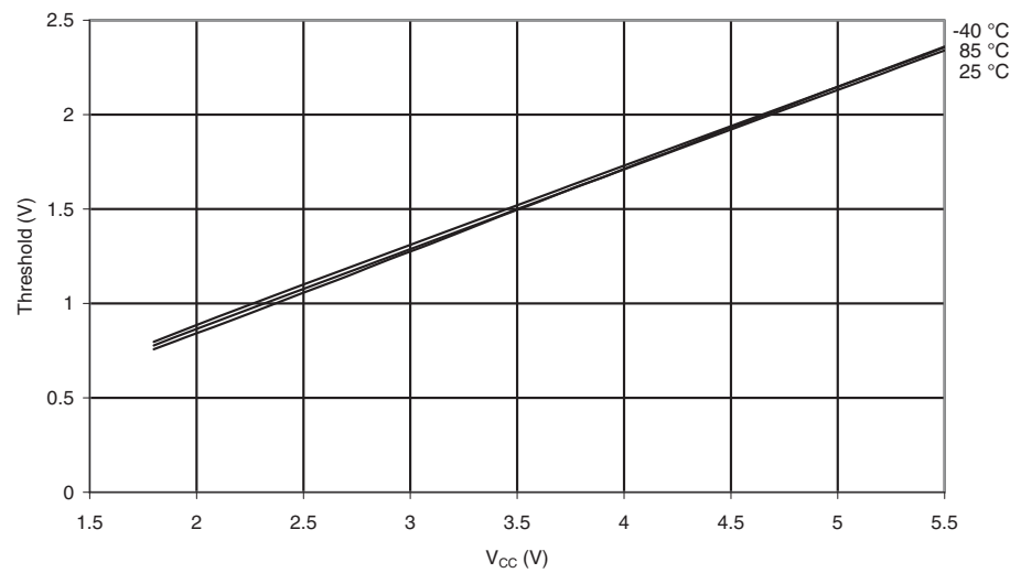
Figure 30-121. Reset Input Threshold Voltage vs. V_{CC} ( V_{IL} , I/O Pin read as '0').
