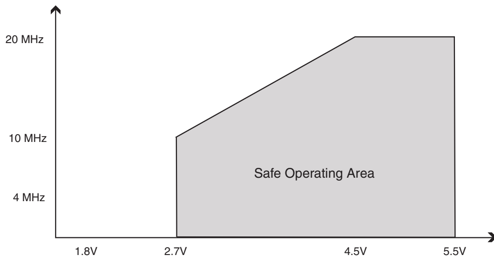
Figure 29-2. Maximum Frequency vs. V_{CC} , ATmega48P/88P/168P
