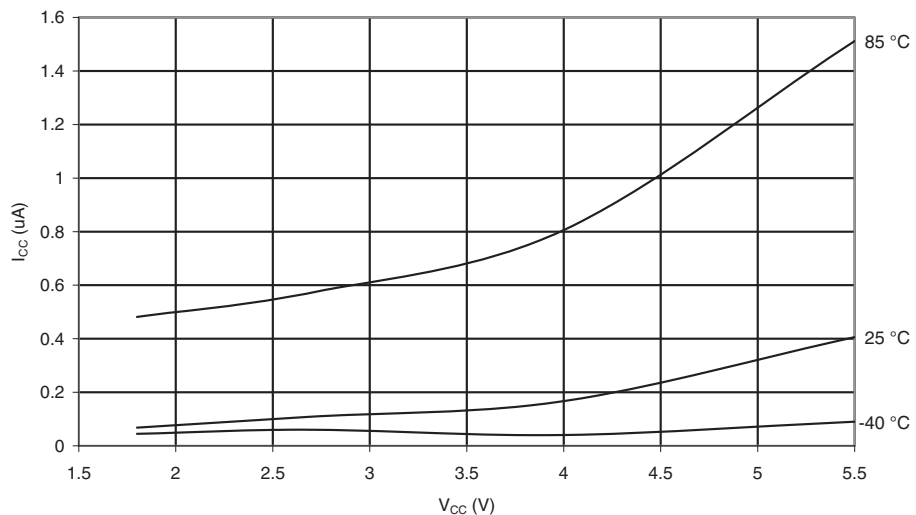
Figure 30-103. Power-Down Supply Current vs. V_{CC} (Watchdog Timer Disabled).
