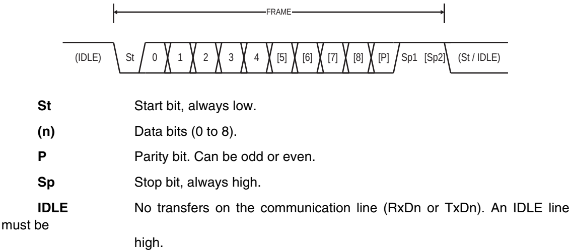
Figure 20-4. Frame Formats
