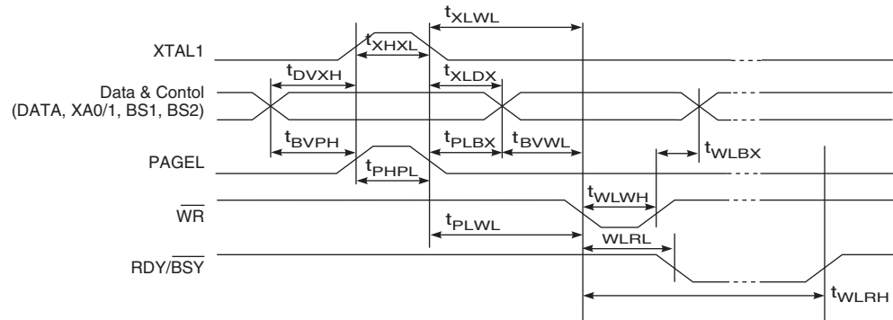
Figure 29-7. Parallel Programming Timing, Including some General Timing Requirements
