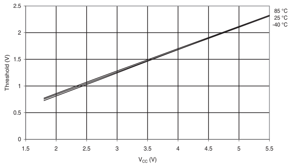
Figure 30-29. Reset Input Threshold Voltage vs. V_{CC} ( V_{IL} , I/O Pin read as '0').
