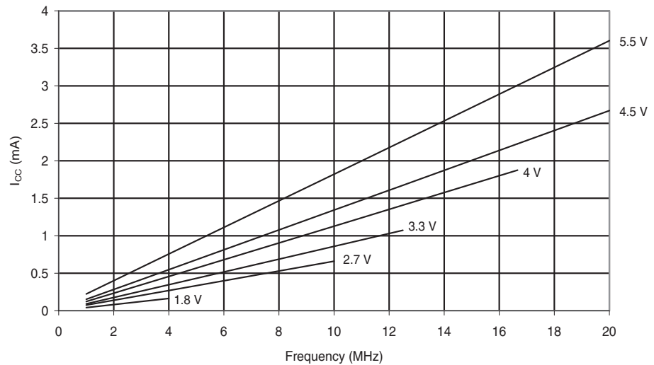
Figure 30-91. Reset Supply Current vs. Frequency (1 - 20 MHz).
