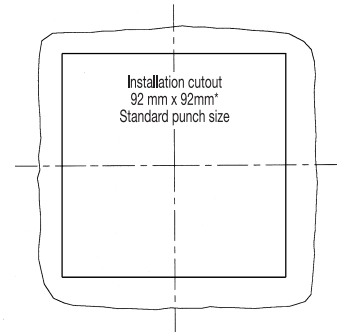
Installation cutout
