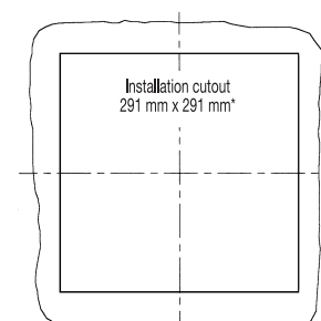
Installation cutout
