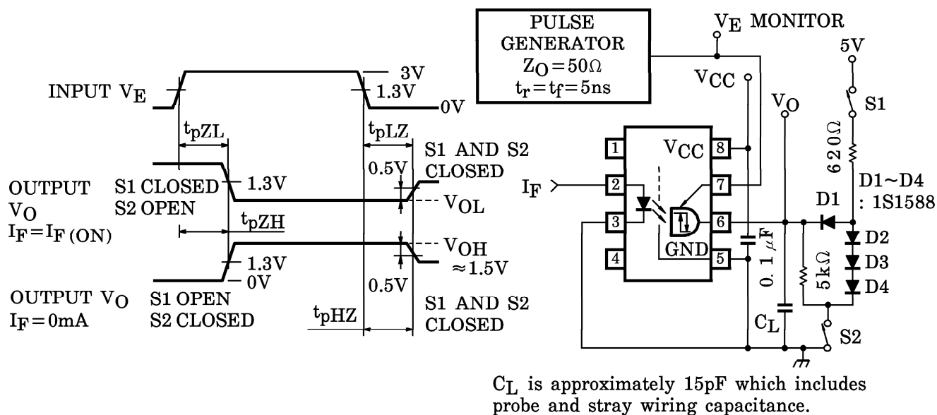
TEST CIRCUIT 2 : t_{pHZ} , t_{pZH} , t_{pLZ} and t_{pZL}
