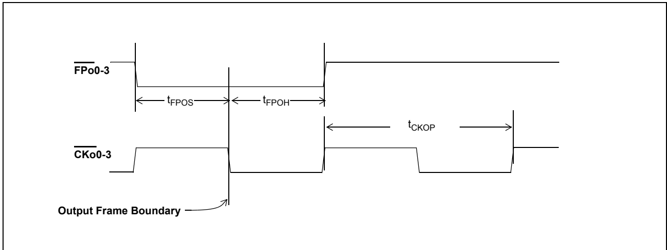
Figure 10 - ST-Bus Frame Pulse and Clock Output Timing
