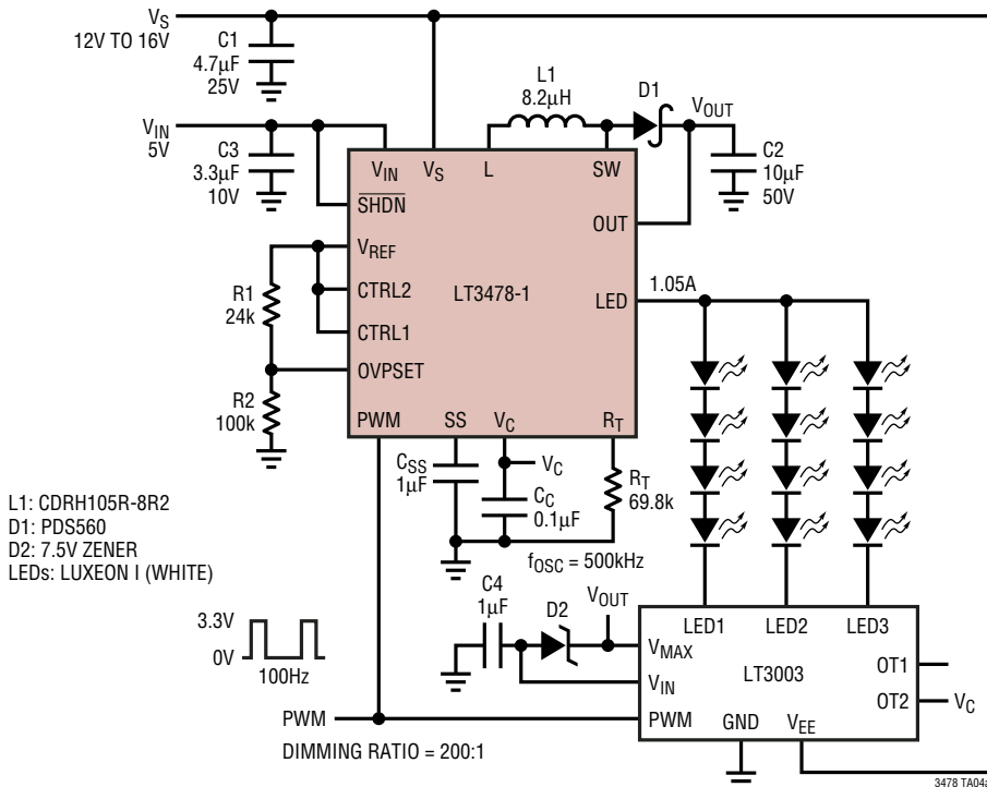
16W, 12 LEDs at 350mA, Buck-Boost Mode LED Driver plus LT3003
