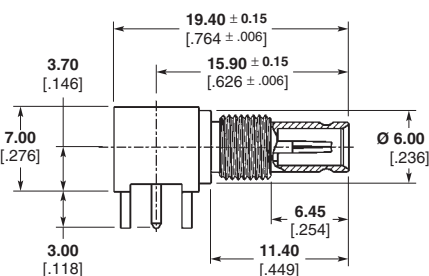
Part Number 1460060-1
