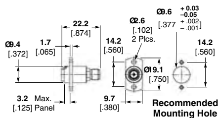
OSP Floating Flange Mount Jack – SMA Jack
