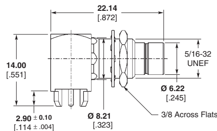
Mounting Detail
