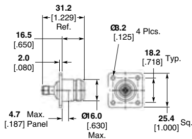
SMA 18 GHz Jack – N Series Flange Mount Jack
