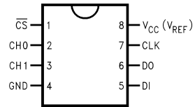
ADC0832 2-Channel MUX Dual-In-Line Package (N)
