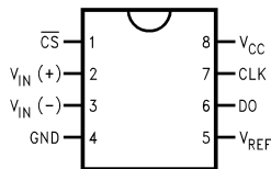
ADC0831 Single Differential Input Dual-In-Line Package (N)
