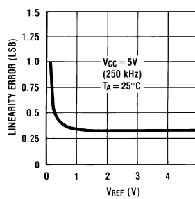
Linearity Error vs V_{REF} Voltage
