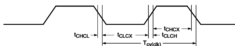
Fig 28. External clock timing (with an amplitude of at least V_{i(RMS)} = 200\text{ mV} )
