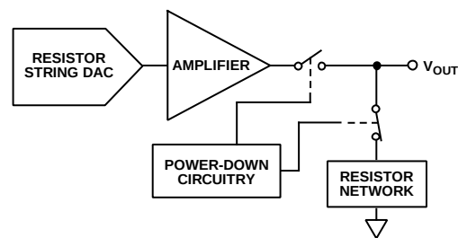
Figure 42. Output Stage During Power-Down
