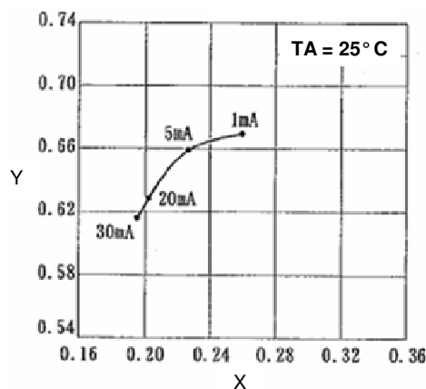
Green: Forward Current vs Chromaticity Diagram
