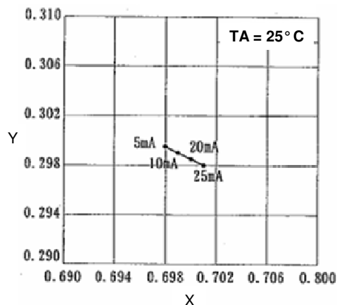
Red: Forward Current vs Chromaticity Diagram
