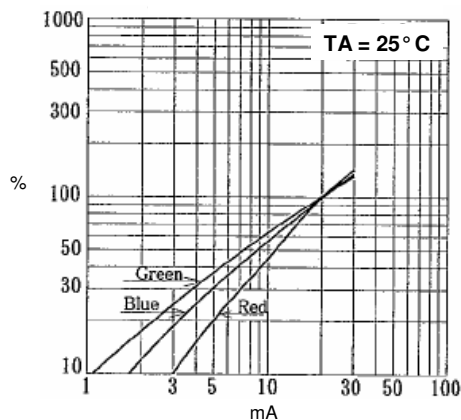
Forward Current vs Relative Luminous Intensity
