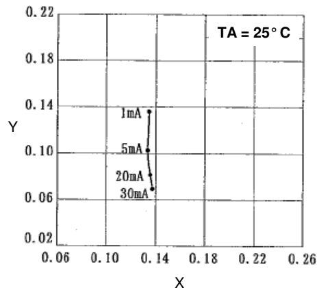
Blue: Forward Current vs Chromaticity Diagram
