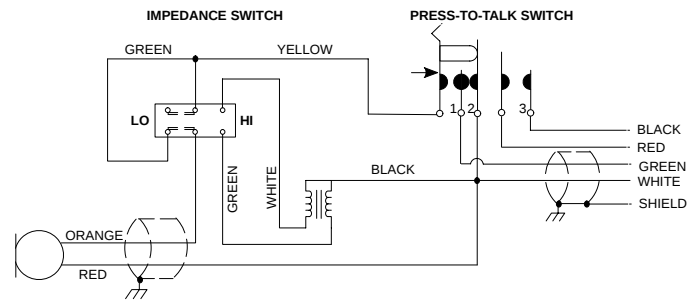
WIRING DIAGRAM
