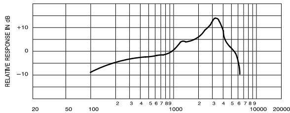
TYPICAL FREQUENCY RESPONSE FIGURE 2
