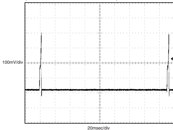
Output Hiccup
