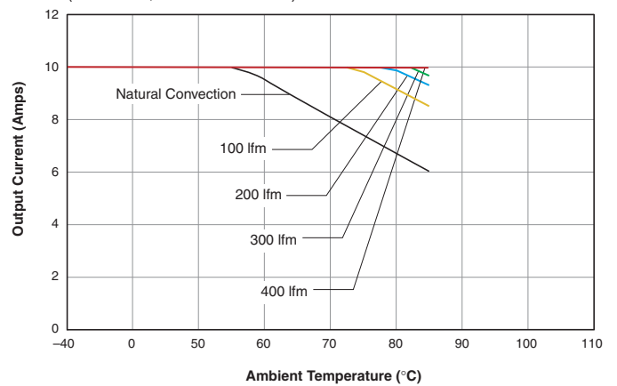
LSM-T/10-D12 Maximum Output Current vs. Ambient Temperature (VOUT = 5V, transverse airflow)
