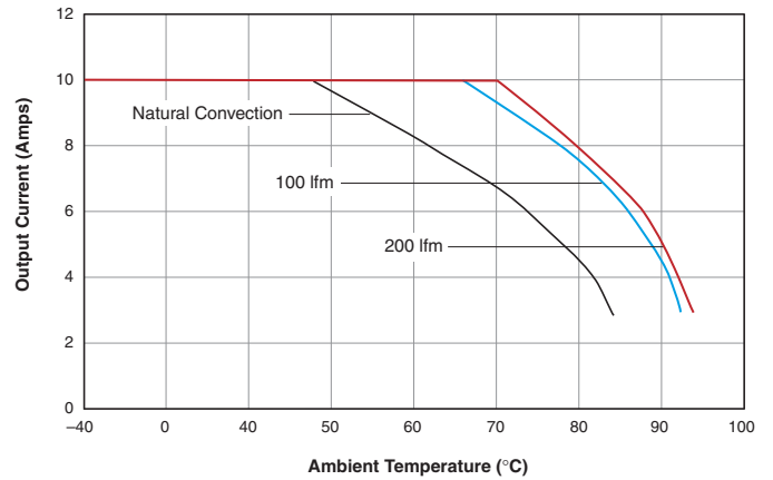
LSM-5/10-D12 Maximum Output Current vs. Ambient Temperature (SMT mount, air flow direction from pin 2 to pin 1)
