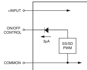
Figure 4A. LSM-T10-D12 Driving the On/Off Control Input
