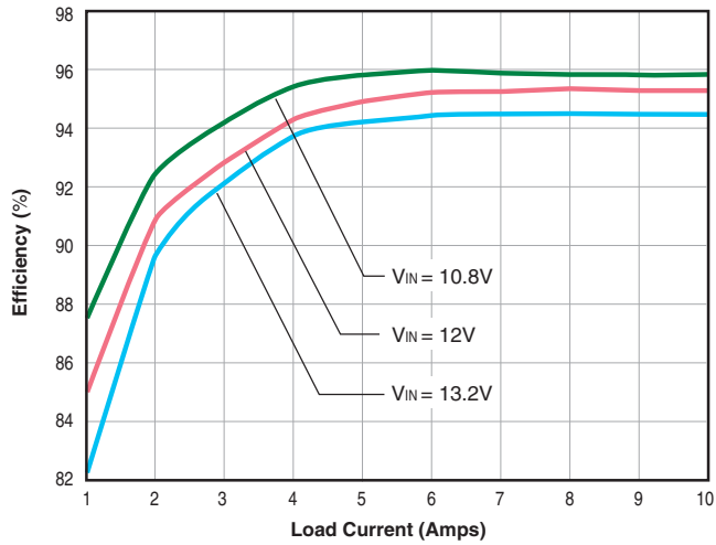
LSM-5/10-D12 Efficiency vs. Line Voltage and Load Current @ +25°C
