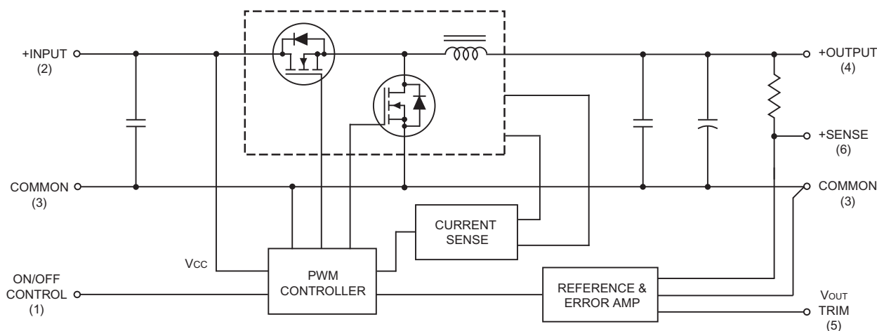
Figure 1. Simplified Schematic
