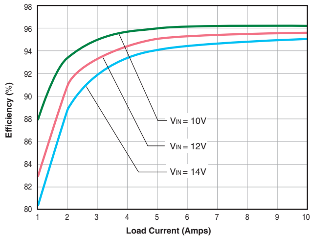
LSM-T/10-D12 Efficiency vs. Line Voltage and Load Current @ +25°C (VOUT = 5V)
