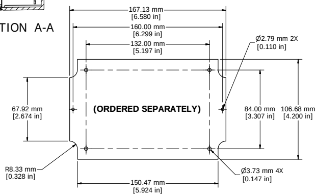
STEEL INNER PANEL
