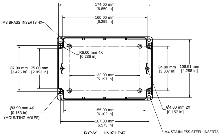
BOX - INSIDE
