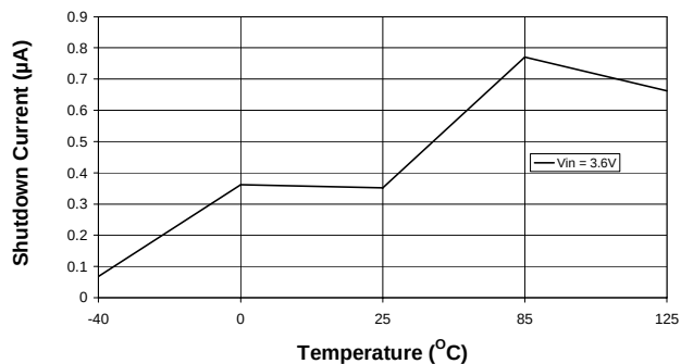
Shutdown Current vs Temperature
