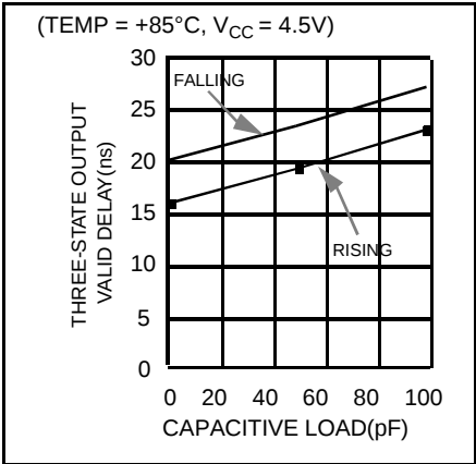
Figure 11. Capacitive Derating Curve
