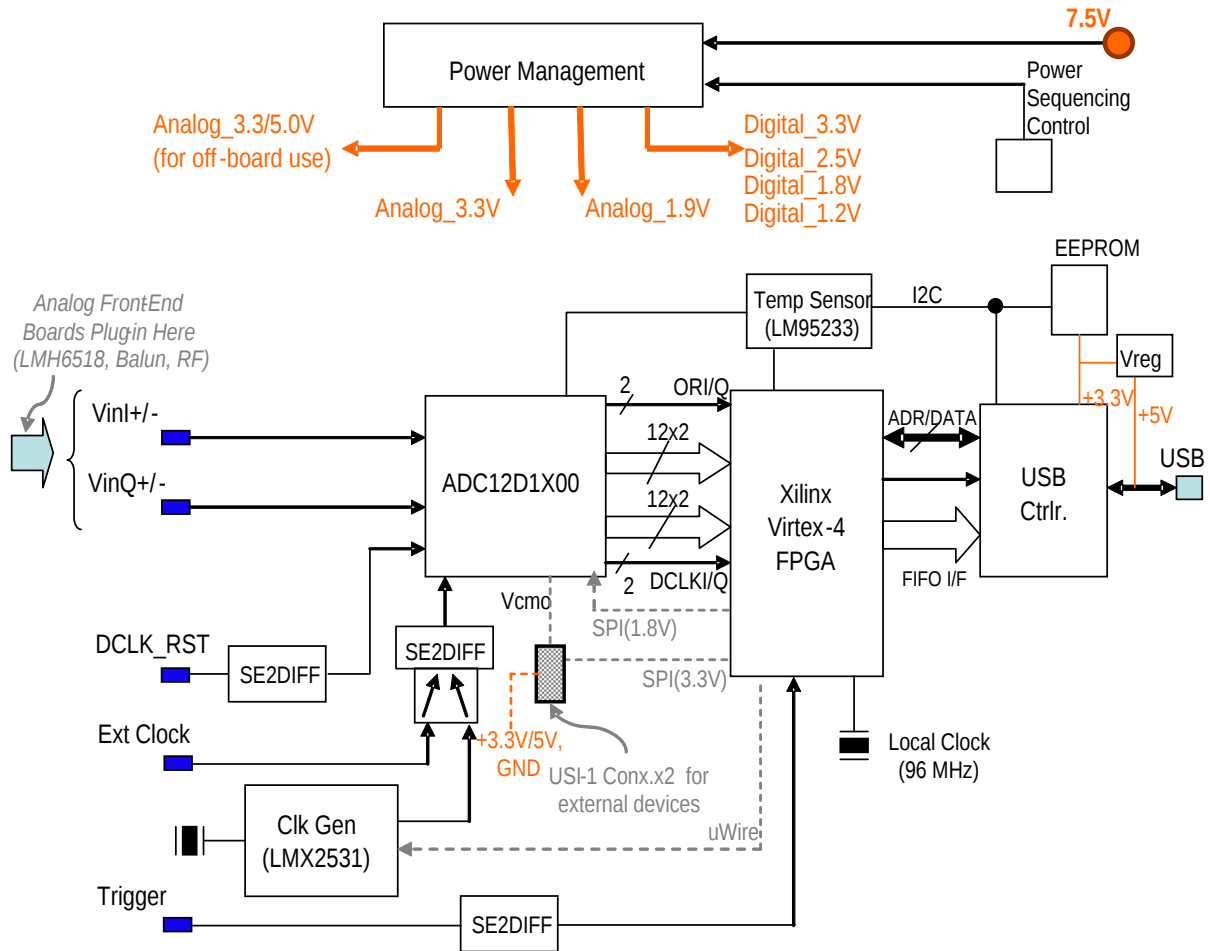
Figure 17: ADC12D1X00RB System Block Diagram
