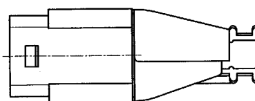
SMS--RDH1 (RECEPTACLE WITH MOULDED ON CABLE HOODS)
