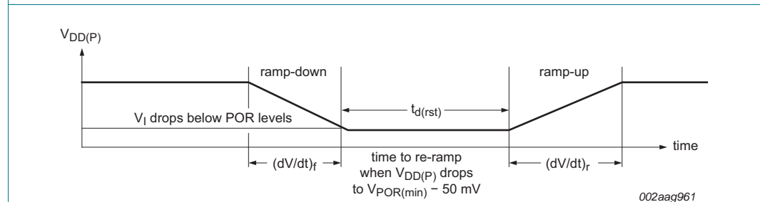
Fig 20. V_{DD} is lowered below the POR threshold, then ramped back up to V_{DD}
