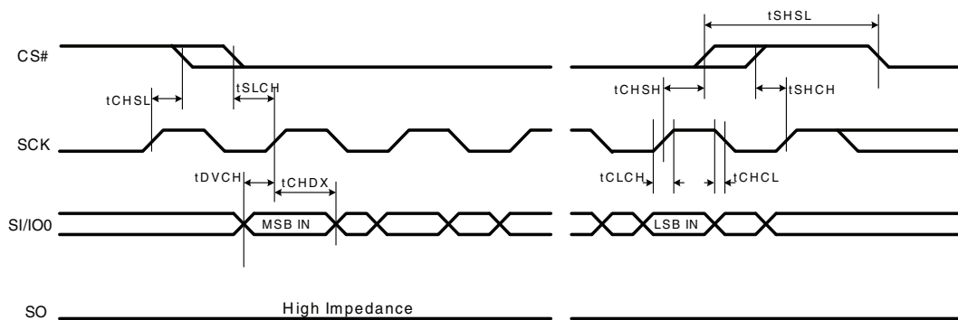
Figure 9.4 Input Timing
