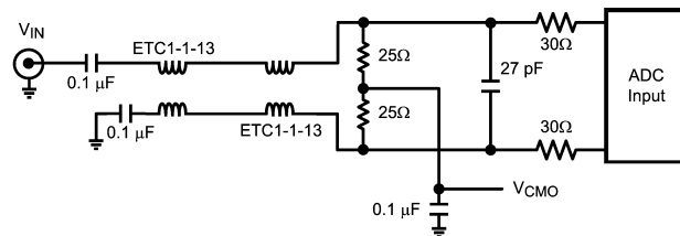
Figure 3. Analog Input Network for F_{IN} > 70\text{MHz}
