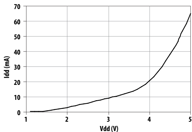
Figure 8. Total Current [1]
