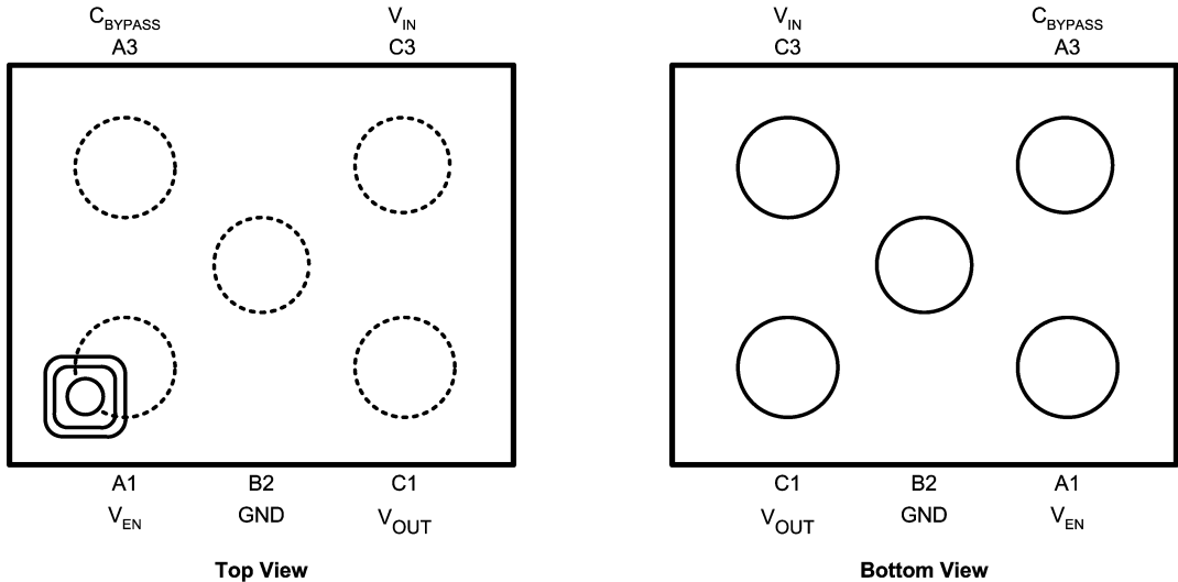
micro SMD, 5 Bump Package
