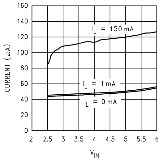
Ground Current vs V_{IN} @ -40^\circ C
