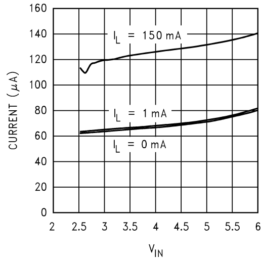
Ground Current vs V_{IN} @ 125^\circ C
