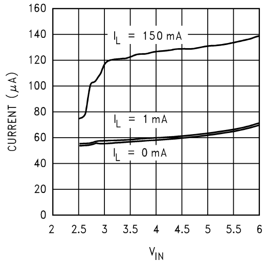
Ground Current vs V_{IN} @ 25^\circ C
