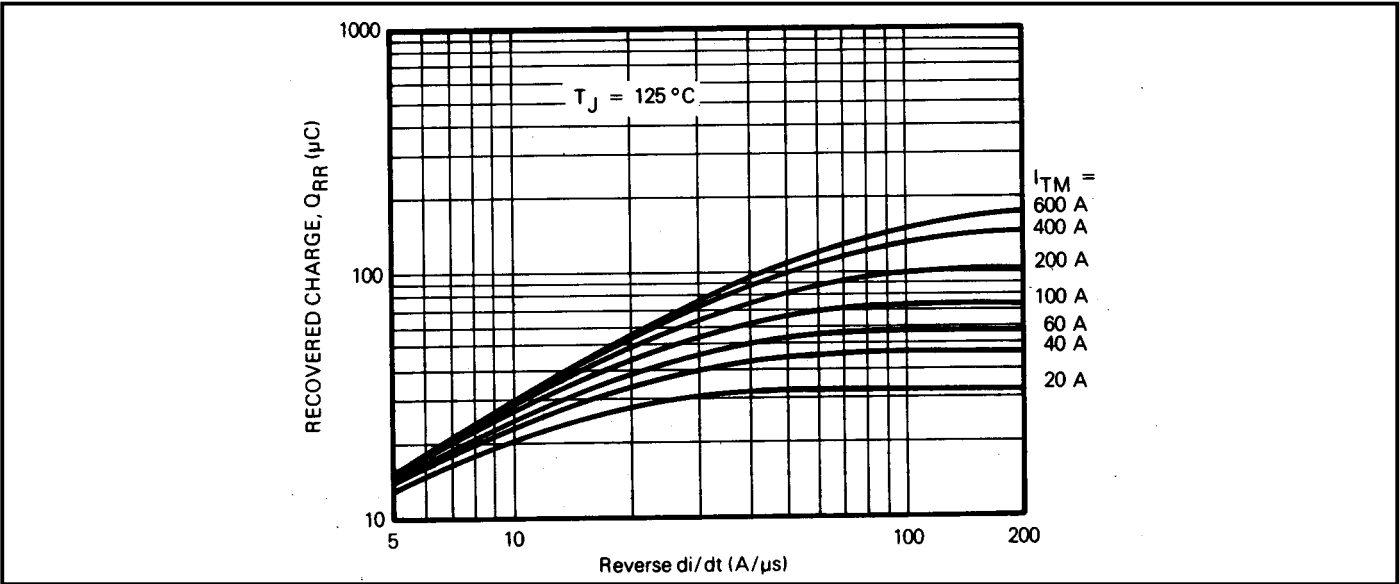
Fig.4 Typical recovered charge (for a device rated V_{DRM} = 600\text{ V} , t_q = 10\mu\text{s} )
