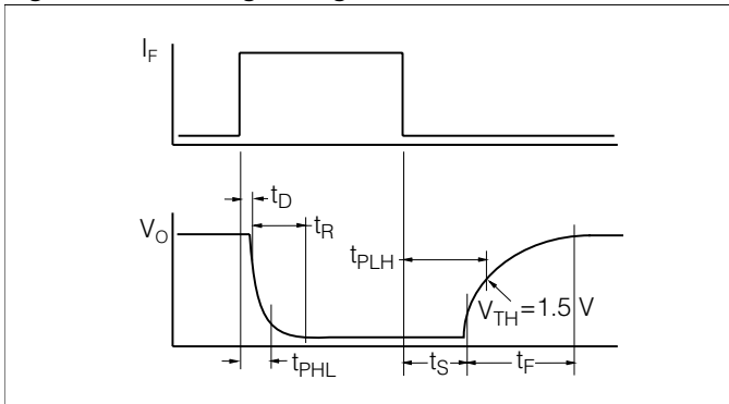
Figure 13. Switching Timing
