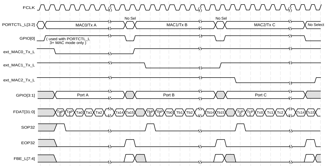
Figure 46. 32-Bit Unidirectional IX Bus Timing - Consecutive Transmits with Prepend, EOP
