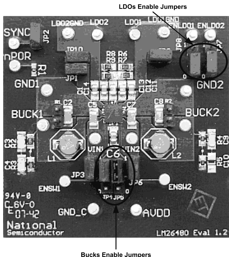
Figure 4. Regulator Enables
