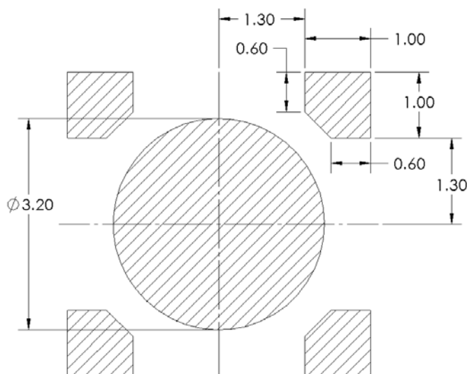
Figure 4: Recommended solder mask opening (hatched area) for anode, cathode, and thermal pad.
