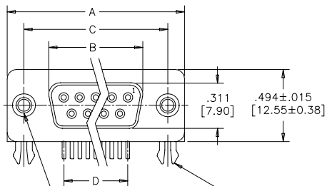
PCB MTG. OPTION C BOARDLOCKS, .318 [8.08] FOOTPRINT
