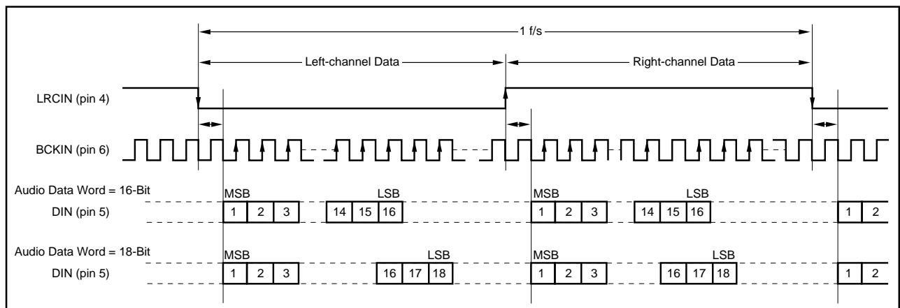
FIGURE 4. "I²S" Data Input Timing.
