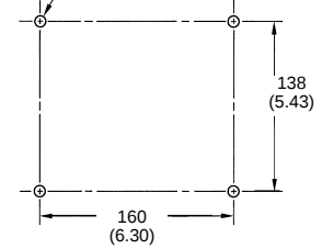
Mounting Holes
