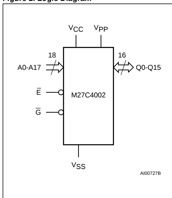
Figure 1. Logic Diagram
