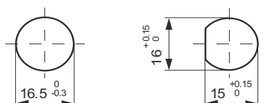
Hole Pattern
