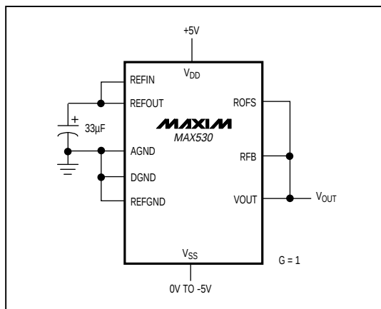
Figure 9. Unipolar Configuration (0V to +2.048V Output)
