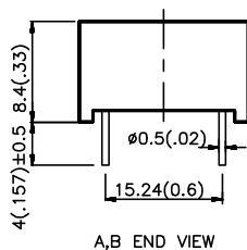
A,B END VIEW
