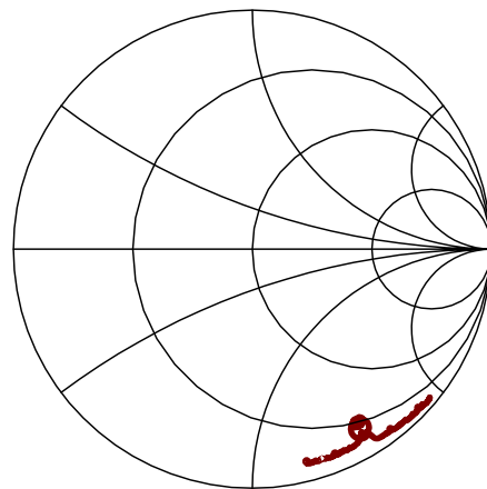
S22 (45-95 MHz)
