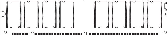
Figure 1: 168-Pin DIMM (MO-161)
