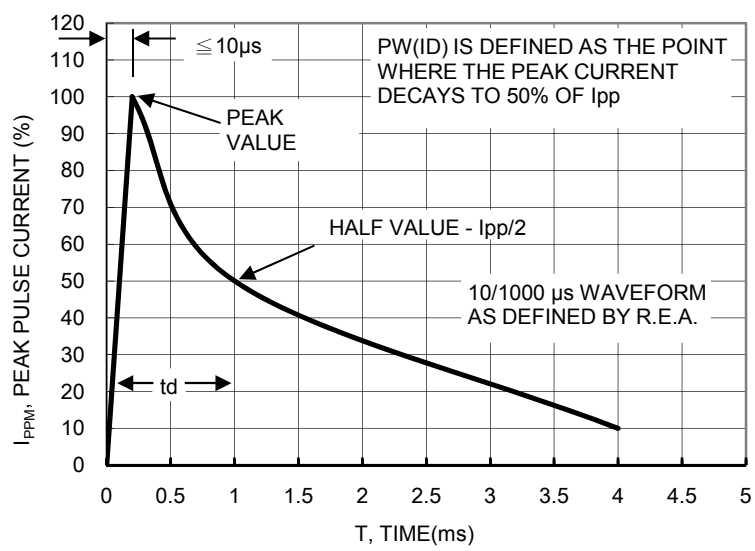
FIG. 7 PULSE WAVEFORM
