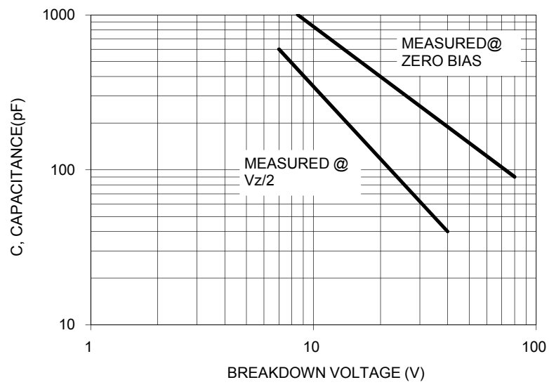
FIG.5 CAPACITANCE CURVE
