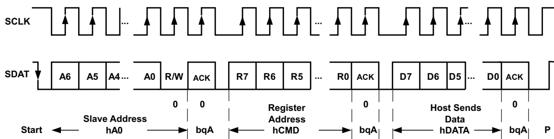
Figure 25. I 2 C read and write operations
