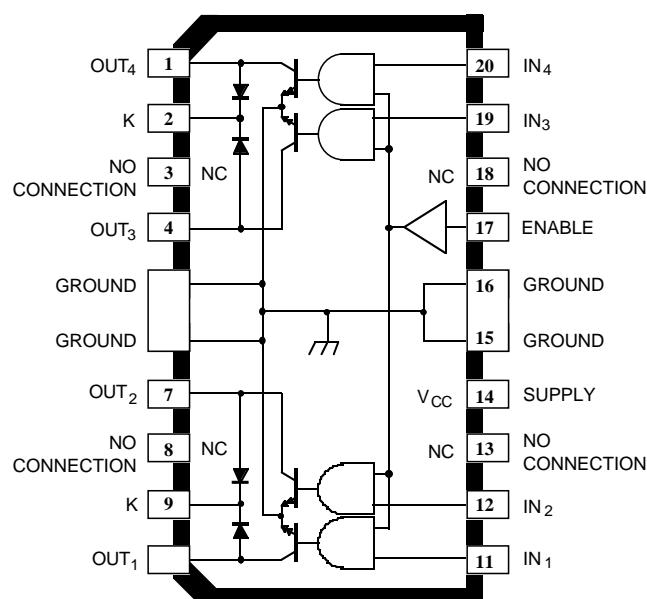
A2540SLB (SOIC)
