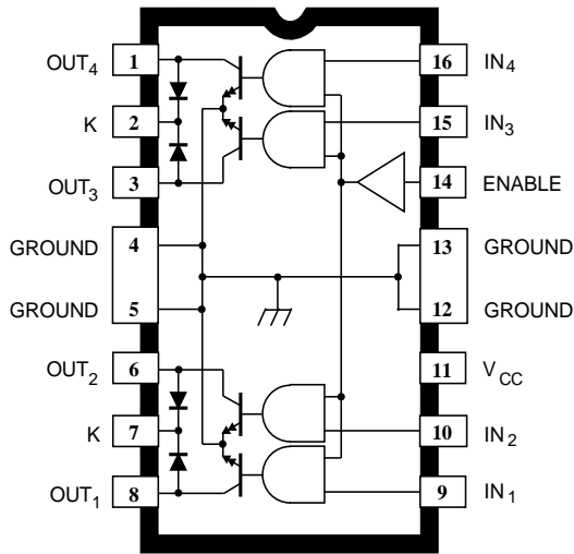
UDN2540B (DIP)
