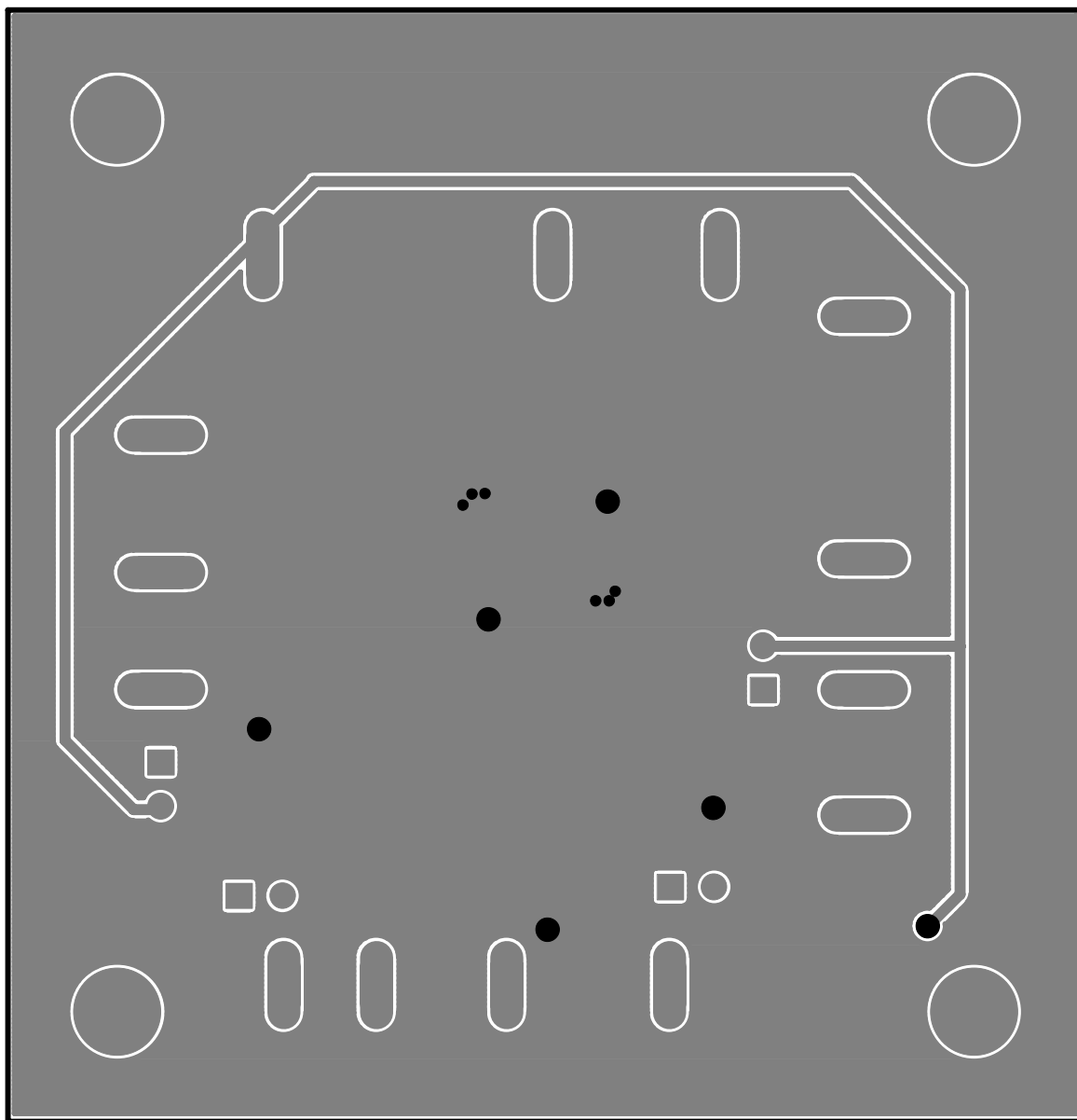
Figure 6. MAX8844Z EV Kit PCB Layout—Solder Side
