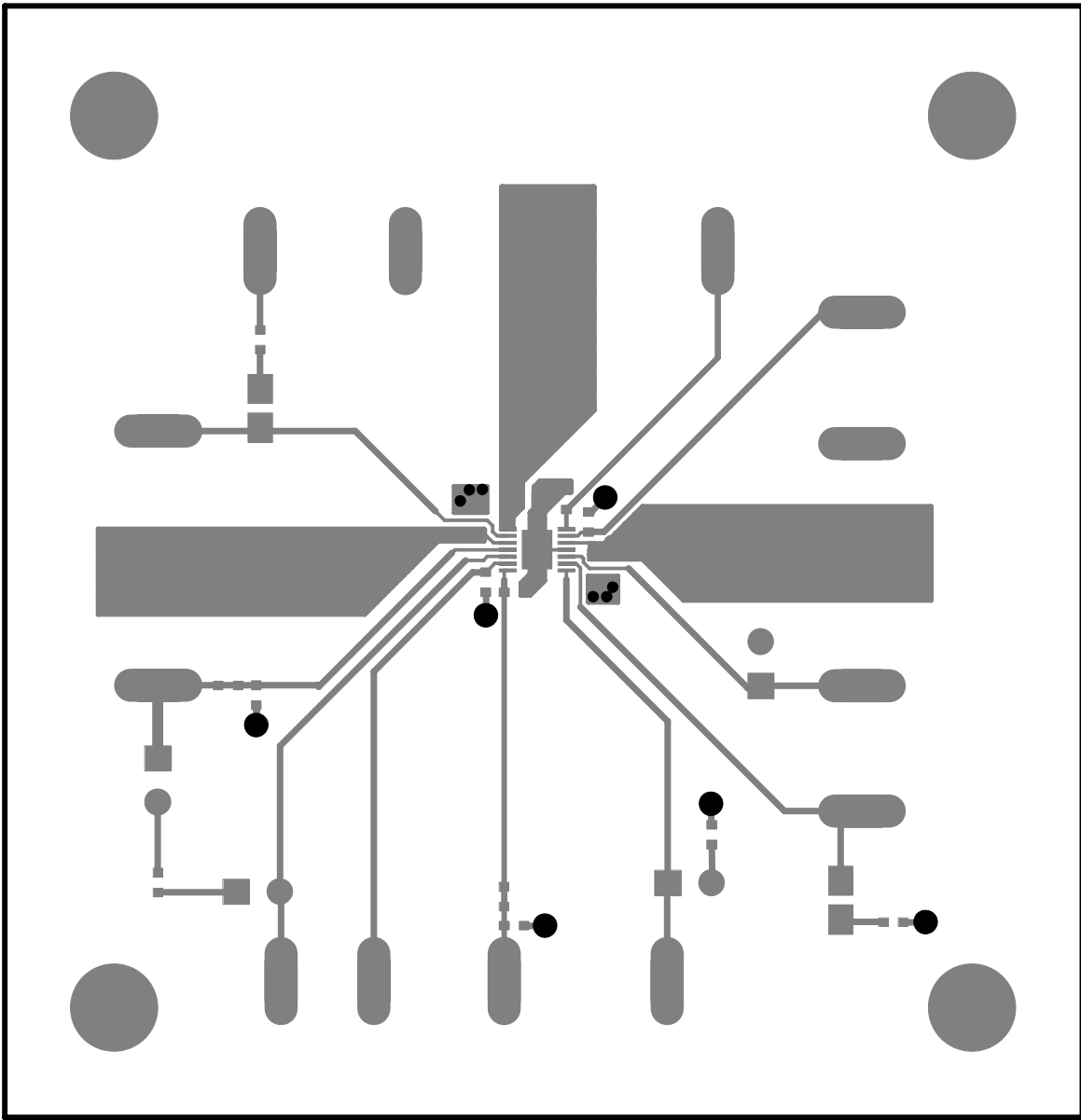
Figure 5. MAX8844Z EV Kit PCB Layout—Component Side
