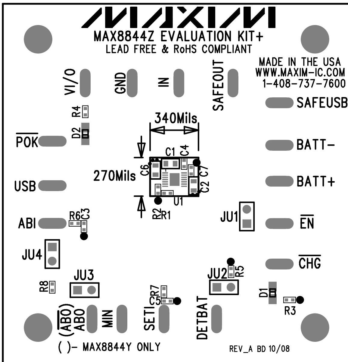
Figure 4. MAX8844Z EV Kit Component Placement Guide—Component Side
