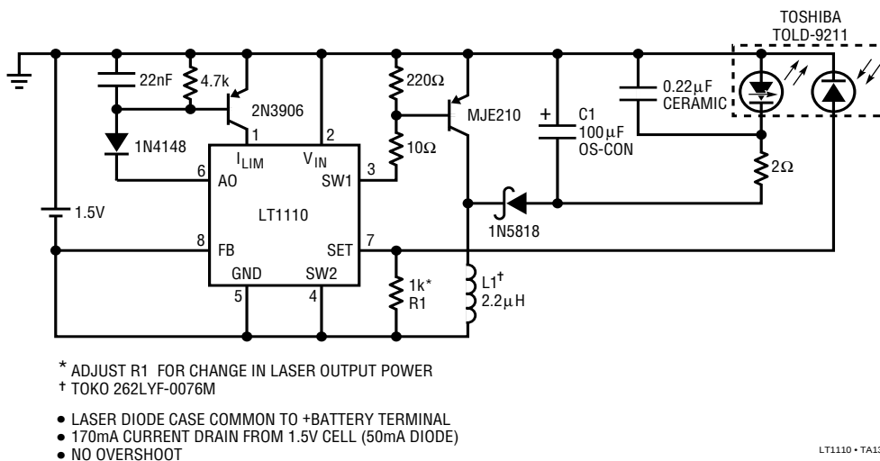
1.5V Powered Laser Diode Driver
