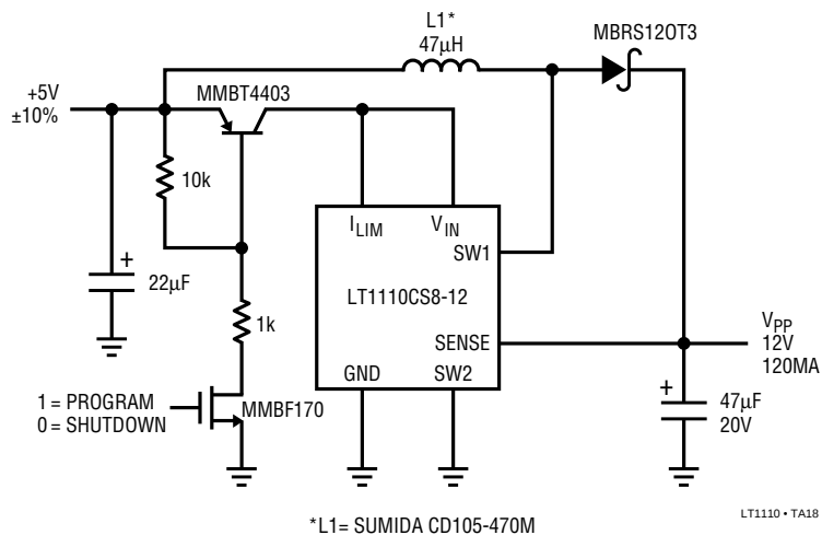
All Surface Mount Flash Memory V PP Generator
