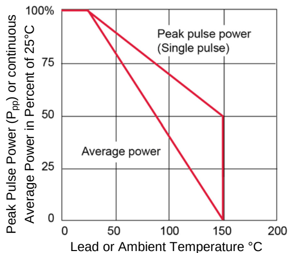
FIGURE 4 Derating Curve
