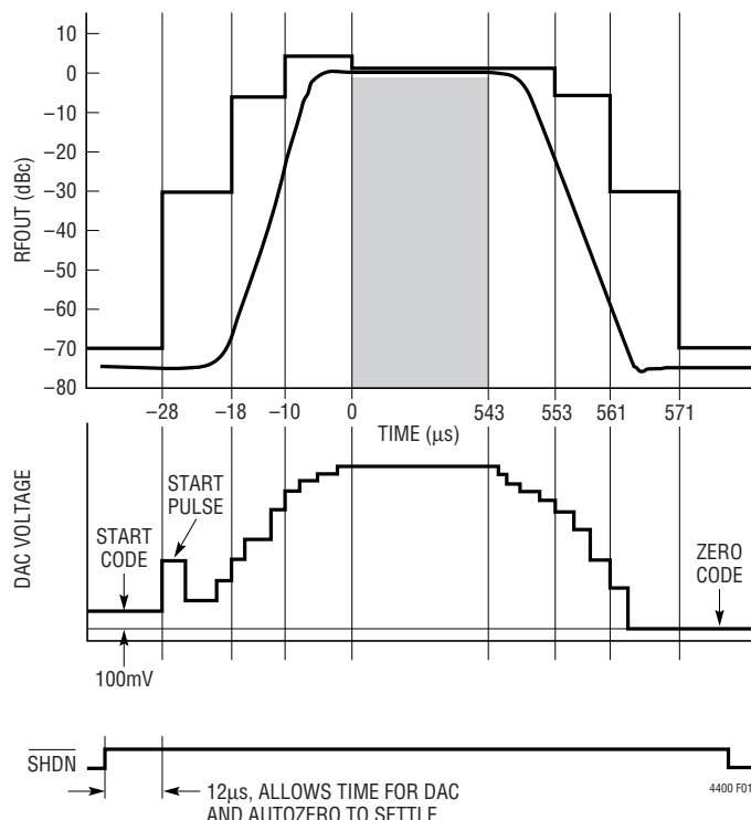
Figure 1. LTC4400-X Ramp Timing
