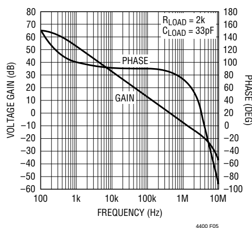
Figure 5. SPICE Model Open-Loop Gain and Phase Characteristics from RF to V_{PCA} , P_{CTL} < 80\text{mV}
