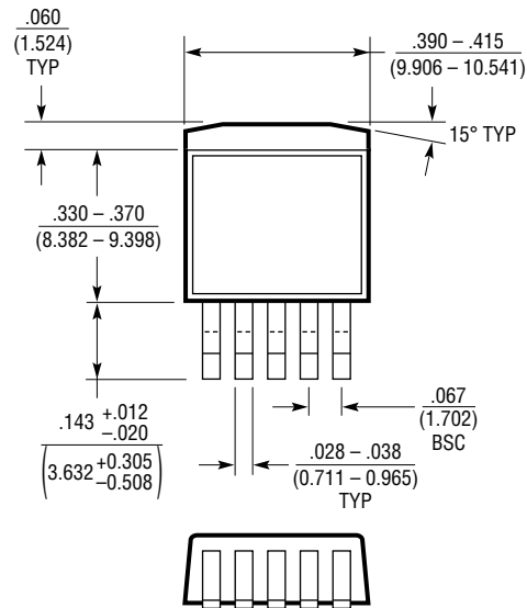
Q Package 5-Lead Plastic DD Pak (Reference LTC DWG # 05-08-1461 Rev F)
